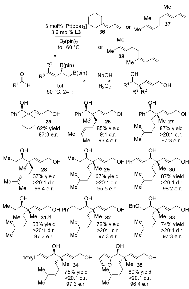
Scheme 3. Asymmetric allylboration of carbonyl groups with \gamma,\gamma -disubstituted allylboronates. Diboration reaction carried out at 60 °C for 12 h with ligand L3 and with [substrate] = 1.0 M in toluene. Allylations were conducted at 60 °C for 24 h with 1 equiv of aldehyde relative to diene and B_2(\text{pin})_2 . Oxidation conducted with 30% H_2O_2 and 3 M NaOH for 4 h. Yield is that of purified material (average of two experiments). Enantiomer ratio determined by HPLC or SFC analysis employing a chiral stationary phase. [a] Used 3 equiv of i\text{PrCHO} .
