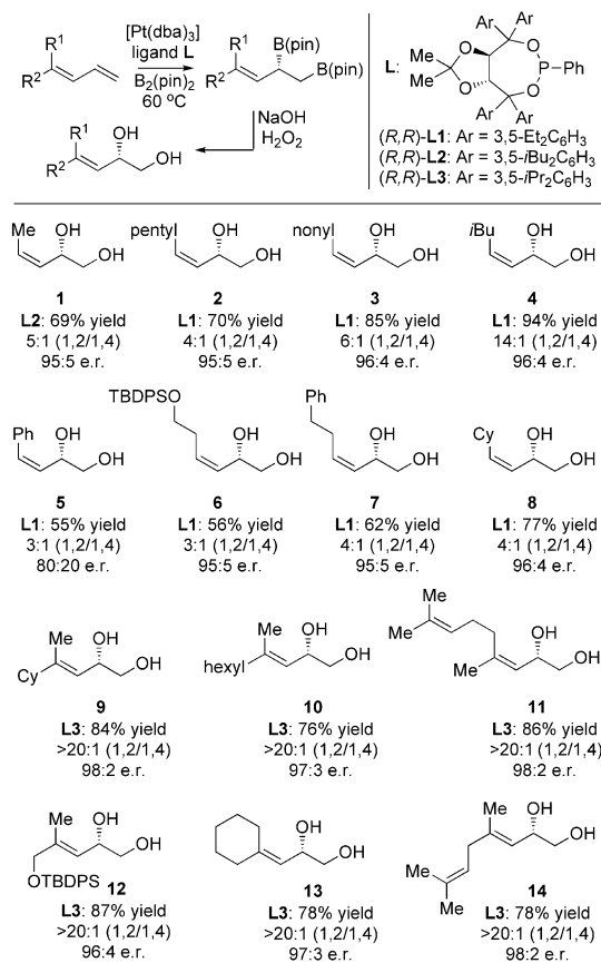
Scheme 2. Catalytic enantioselective 1,2-diboration of 1,3-dienes. Reactions carried out at 60 °C for 12 h, with subsequent oxidation using 30% H 2 O 2 and 3 M NaOH for 4 h. For products 1–8 , 3 mol % of [Pt(dba) 3 ], 6 mol % of ligand, and THF were employed. For products 9–14 3 mol % of [Pt(dba) 3 ] and 3.6 mol % of ligand employed. Yield is that of the purified 1,2-diol (average of two experiments). Enantiomeric purity determined by GC analysis of a derivative employing a chiral stationary phase (see the Supporting Information for details). dba = di-benzylideneacetone, pin = pinacol, TBDPS = tert -butyldiphenylsilyl.
