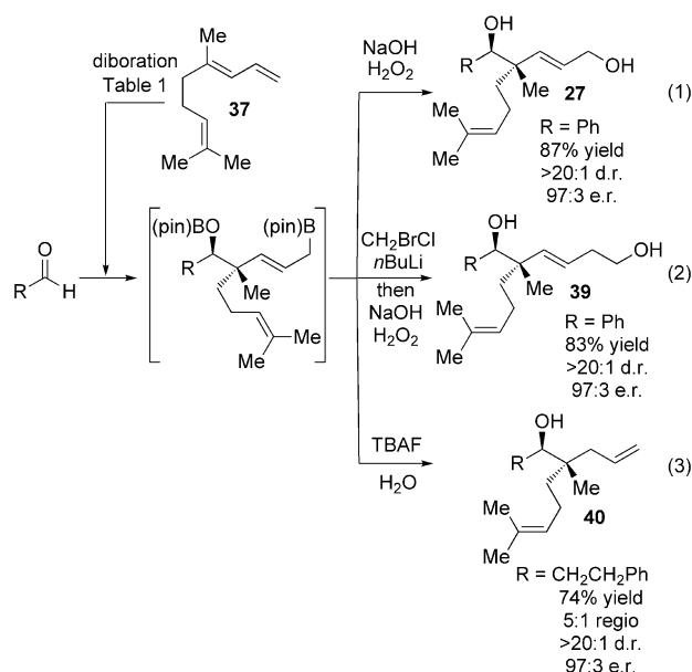
Scheme 4. Diboration/allylation/functionalization sequence. TBAF = tetra- n -butylammonium fluoride.
